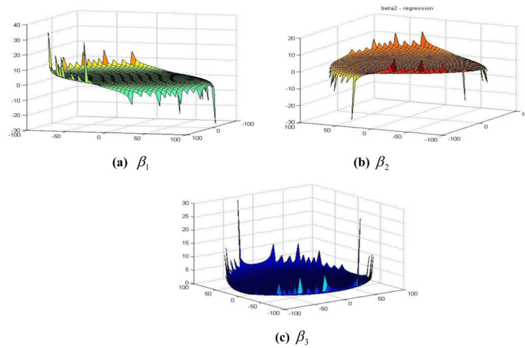
Figure 2. Variation shapes of bias in estimation for the three coefficients X1, X2 and X3 when both r1 and r2 vary from -1 to 1 . The figures show how the estimates of \beta_1 , \beta_2 , and \beta_3 vary according to different conditions of two correlation coefficients between the correlation coefficient between X1 and X2 ( r_1 ) and the correlation coefficient between X1 and X3 ( r_2 ): (a) for \beta_1 , (b) for \beta_2 , and (c) for \beta_3 . The X-axis represents r_1 , Y-axis is r_2 , and Z-axis is the regression coefficient.
